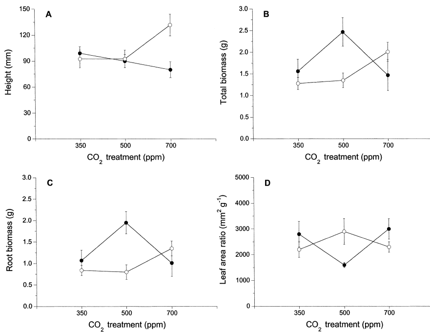
Figure 2. Mean ( \pm 1 SE) height (A), total biomass (B), root biomass (C), and leaf area ratio (D) of Q. cerrroides (filled dots) and Q. ilex (hollow dots) seedlings according to the different levels of atmospheric CO 2 enrichment.
