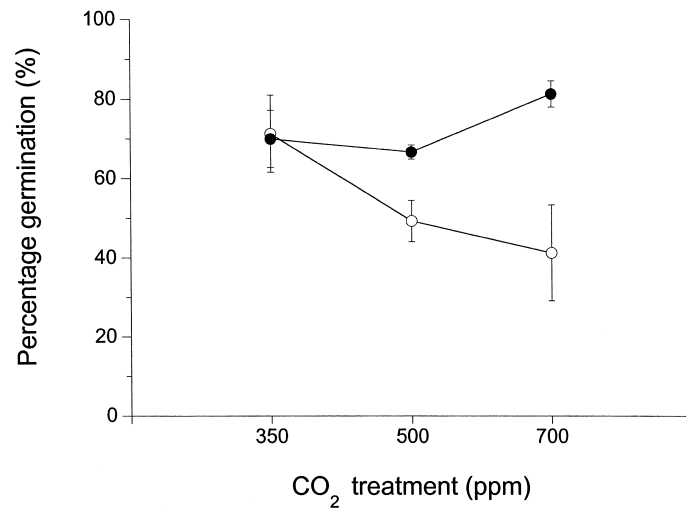
Figure 1. Mean ( \pm 1 SE) percentage germination of Q. cerrroides (filled dots) and Q. ilex (hollow dots) according to the different levels of atmospheric CO 2 enrichment.
